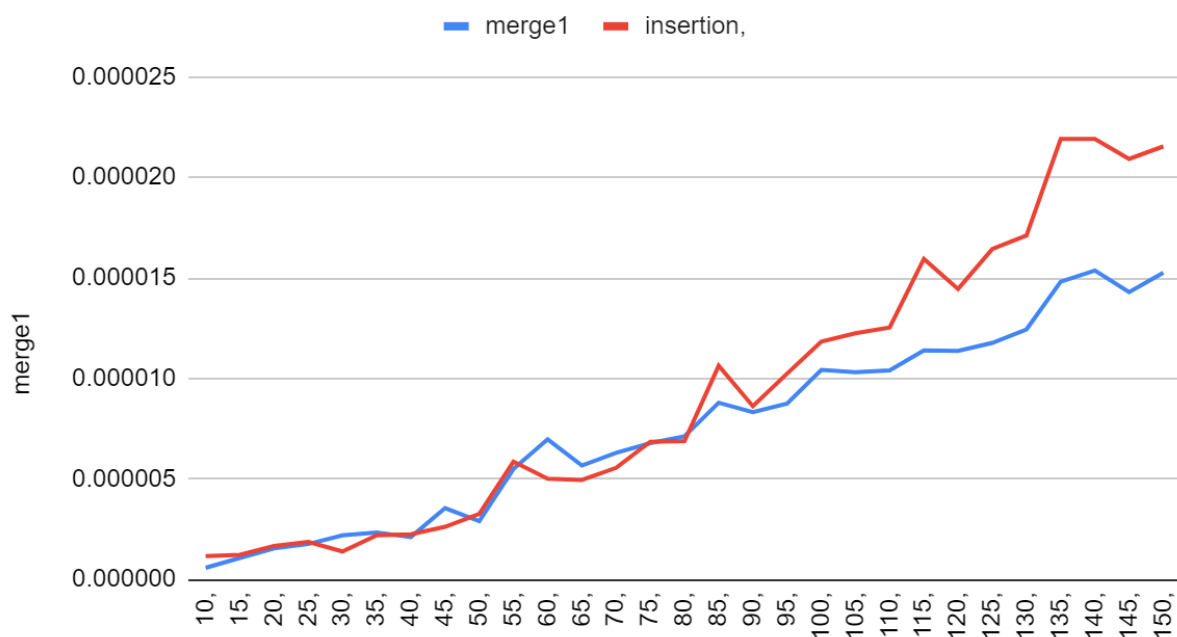
merge1 vs. insertion,
